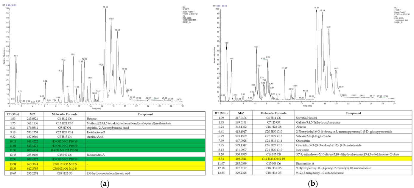
Figure 6. Chromatogram of ethanol-based solvent S. caseolaris leaves extract: (a) run A; (b) run B. Upper panels are chromatogram of LC-MS/MS data and lower panels are list of identified compounds.
