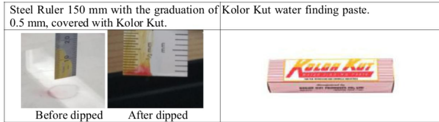
Figure 7. Steel ruler with Kolor Kut to measure the water depth.
