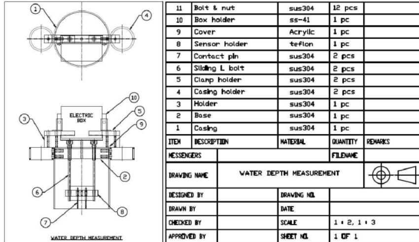
Figure 2. Design drawing for a measuring device.
