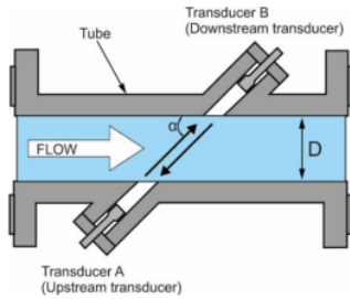
Fig. 4. Ultrasonic transit time flow meter.
