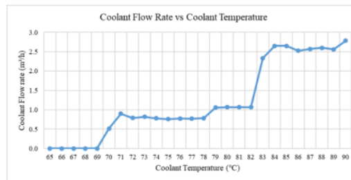
Fig. 9. Engine coolant flow rate as a function of engine temperature.
