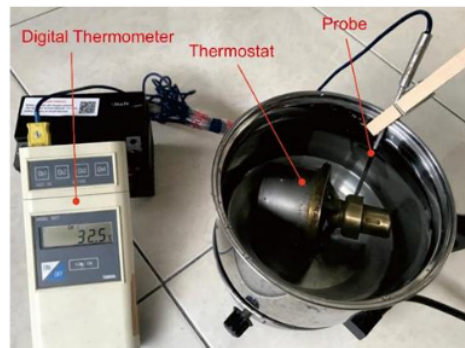
Fig. 6. Preparatory conditions for thermostat character testing.
