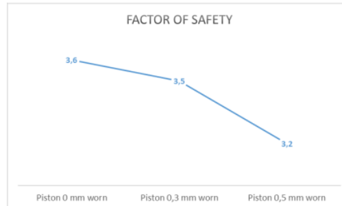
Fig. 5. Factor of safety result
