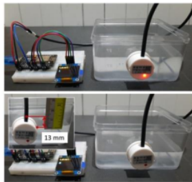
Fig. 6. Level sensor working test and position setting.
