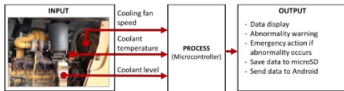
Fig. 2. Input, process, and output diagram.
