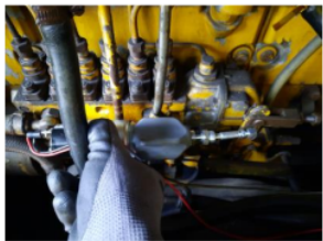
Fig. 16. Fuel solenoid placement.
