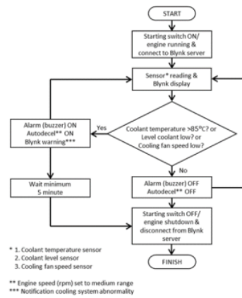
Fig. 3. Monitoring and warning flow diagram.
