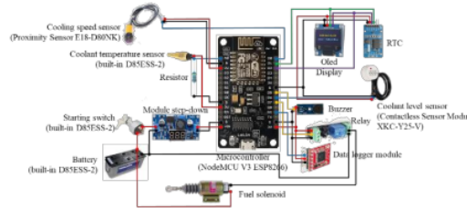
Fig. 4. Device block diagram.
