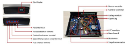
Fig. 8. Front, back, and inside box view.
