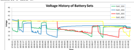
Figure 7: History of each group battery voltage after 18:00.
